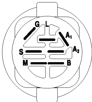
IGNITION SWITCH
